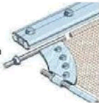
Extruded section with membrane plate and centenary cables
